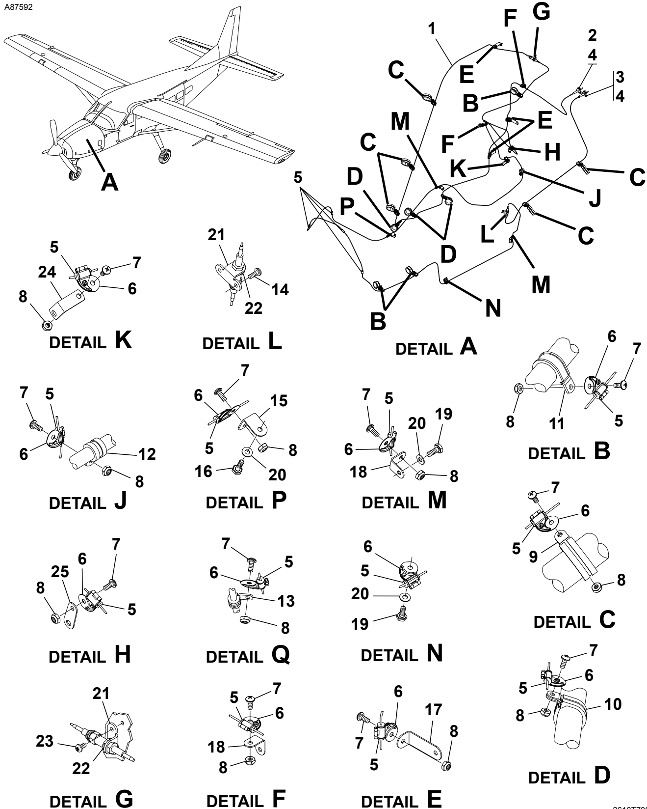
FIRE DETECTION SYSTEM Figure 02. (Sheet 1)
