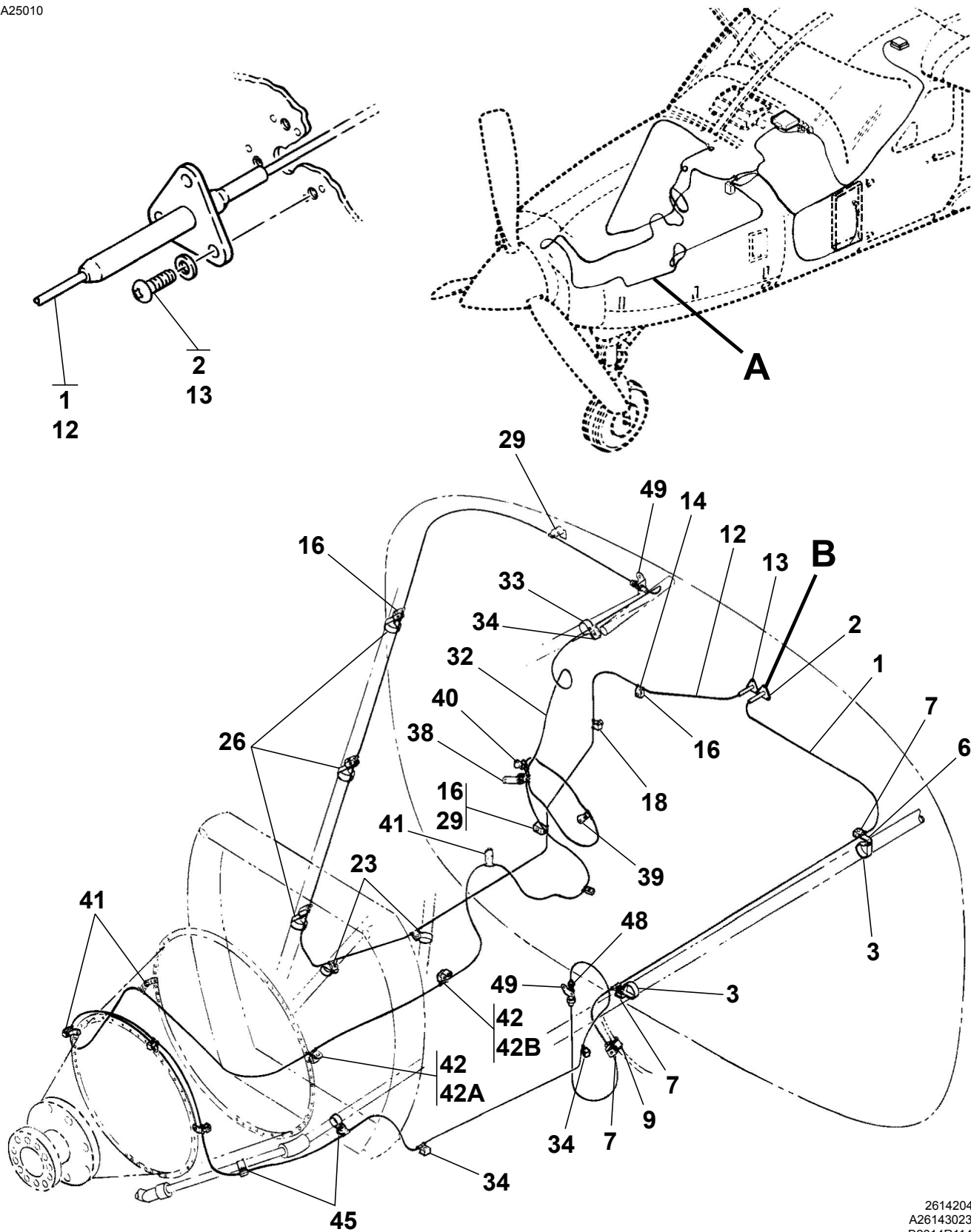
FIRE DETECTION SYSTEM Figure 01. (Sheet 1)
