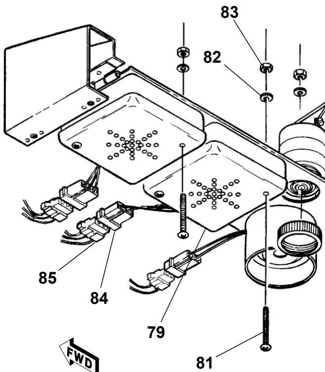
DETAIL B
