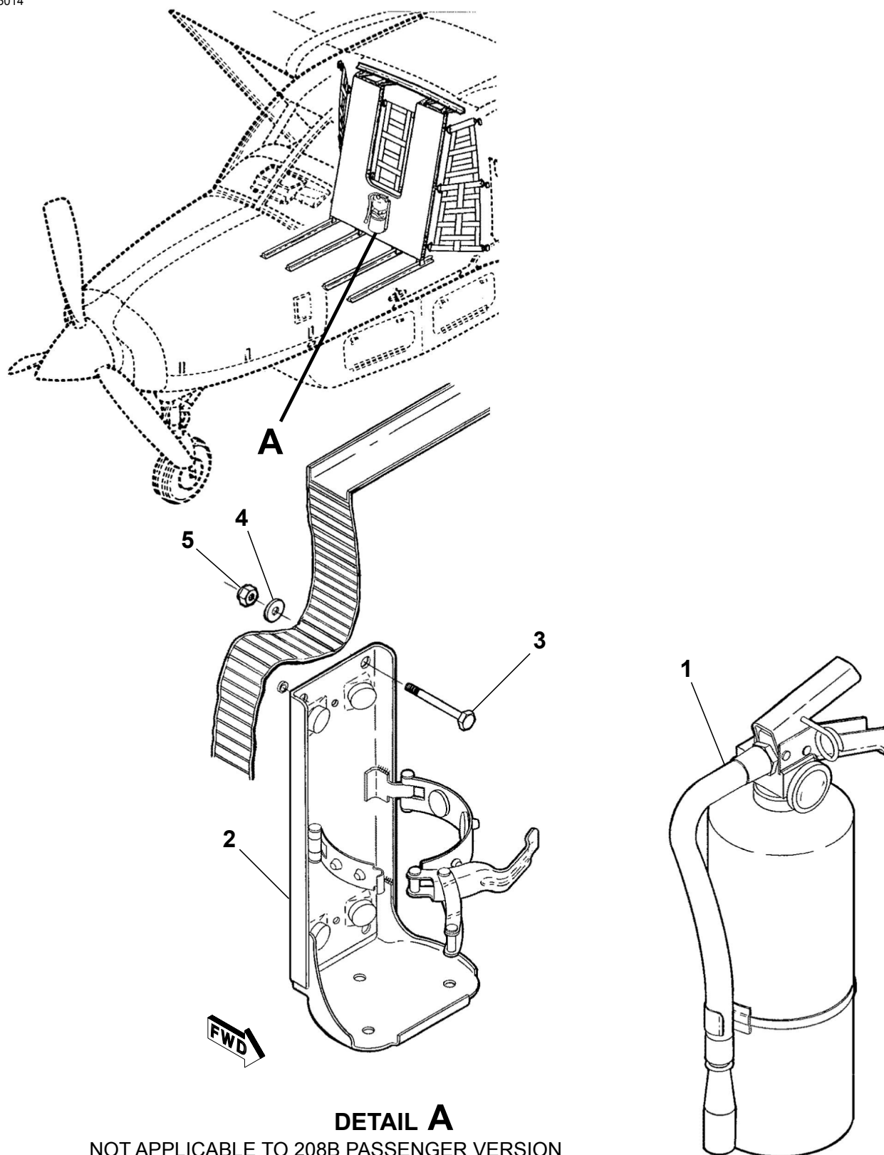
FIRE EXTINGUISHER INSTALLATION Figure 01. (Sheet 1)
