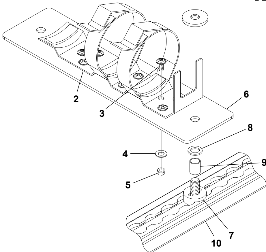
DETAIL B
